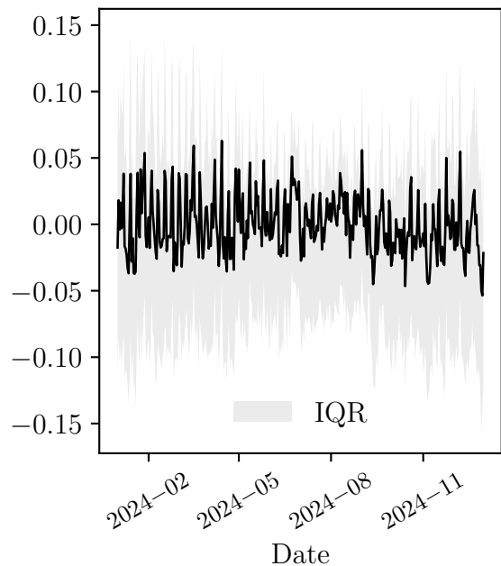
Mean residuals
